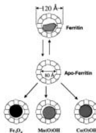
Figure 1. A schematic of the synthetic routes to different nanoparticles. A variety of other oxides can be assembled within the protein cage of ferritin (cross-sectional view shown).
